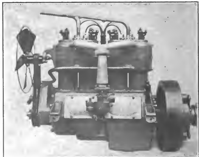
Fig. 2—Left side of the latest Reo motor
